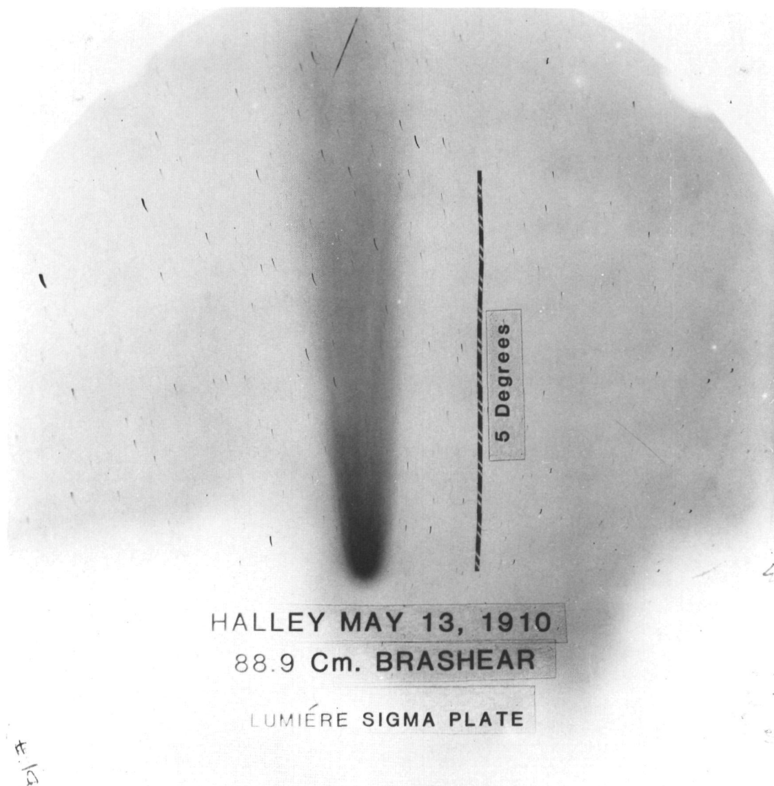
Figure 3. Photograph of Comet Halley obtained on May 13, 1910.
